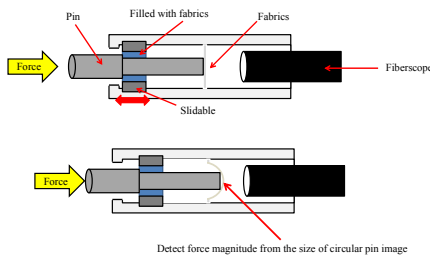
Figure 2. Principle for sensing force in depth direction of endoscope
