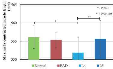
Fig. 8. Maximally contracted muscle length of quadriceps muscle at the reference model
