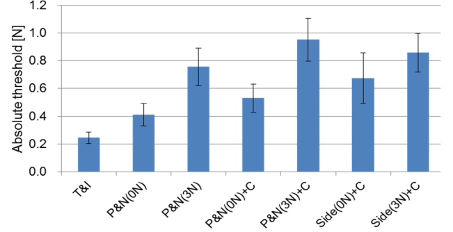
Fig. 9. Obtained absolute threshold of pulling force
