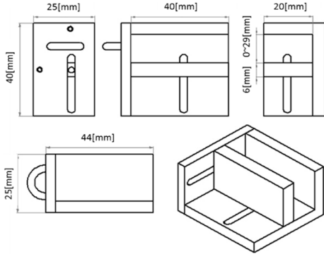
Fig. 6. Fixture for the styles shown in Fig. 3 (b) and (c)
