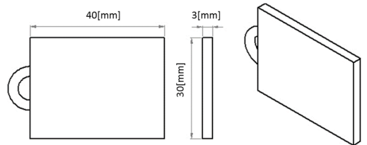
Fig. 5. Plate for the style shown in Fig. 3 (a)
