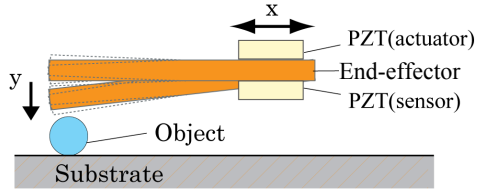
Fig. 8 Displacement induced by DC input
