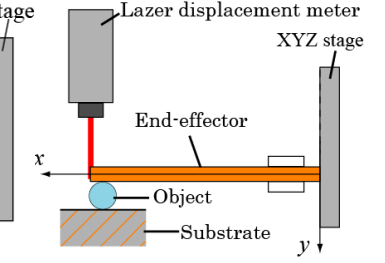
Fig. 5 View of the experiment set up from the microscope side
