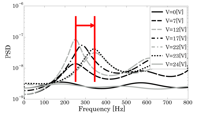
Fig. 11 Shift of target peak frequency
