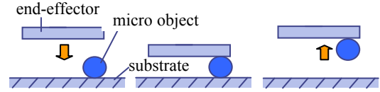
Fig. 1 Micro object adhered to end-effector
