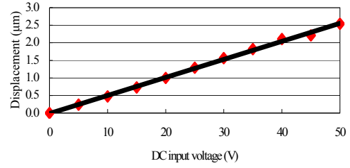
Fig. 9 The relation between DC input voltage and tip displacement
