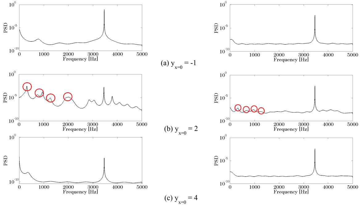
Fig. 6 Experimental results. The left column shows the results obtained by applying FFT to the measured oscillation by laser displacement meter and the right column shows the results obtained by applying FFT to the measured oscillation by the PZT sensor.
