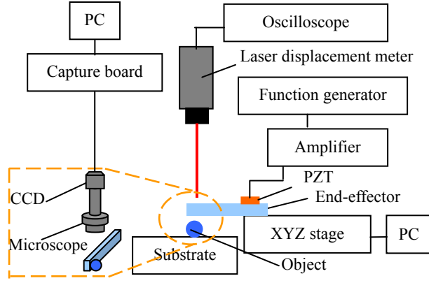
Fig. 3 Overview of the experimental setup
