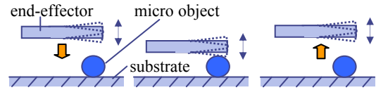
Fig. 2 Relaxation of adhesion force
