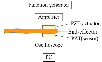
Fig. 7 Overview of the hybrid actuator and sensor system
