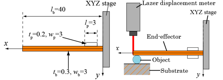
Fig. 4 End-effector and the coordinate.
