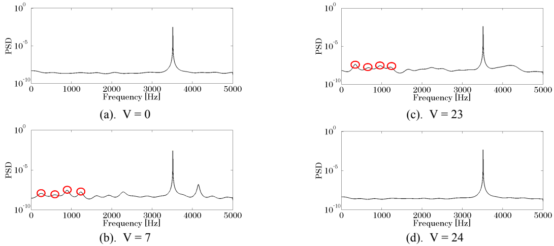
Fig. 10 Experimental results obtained by applying FFT to the induced voltage at the PZT sensor when adding the combined input of the DC and the AC inputs to the PZT actuator.
